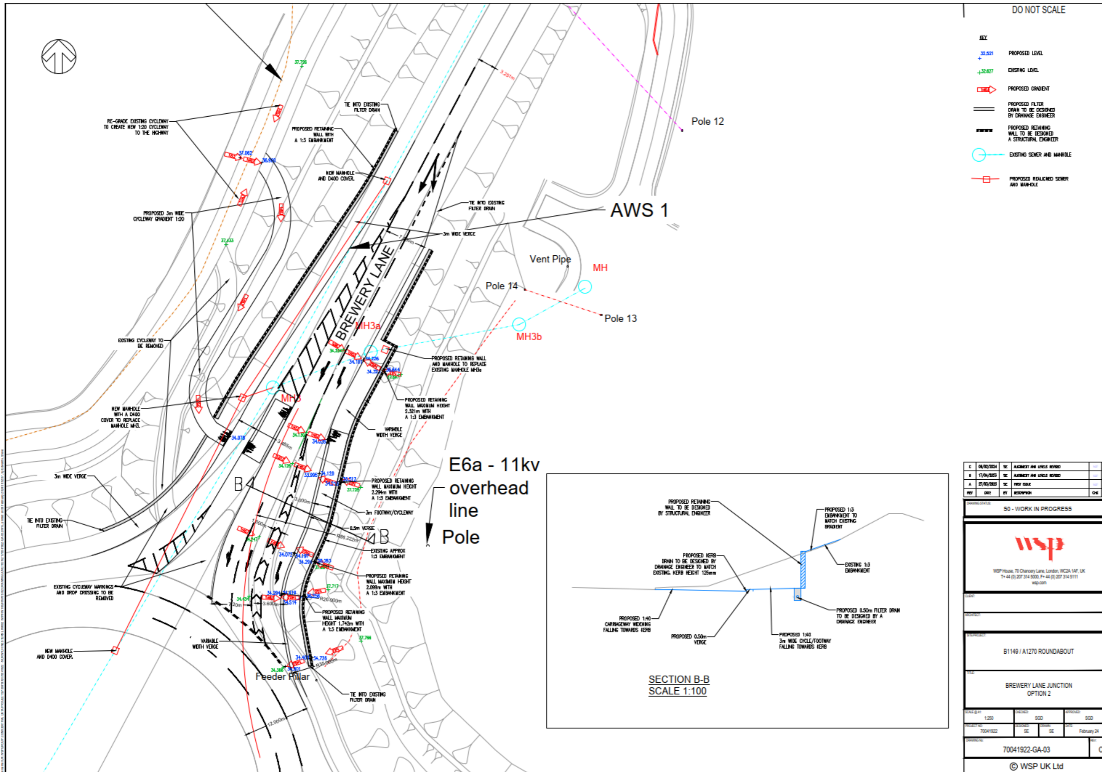
Figure 1 A1270/Brewery Lane Junction - Northern Arm Emerging NCC Capacity Enhancement Scheme
