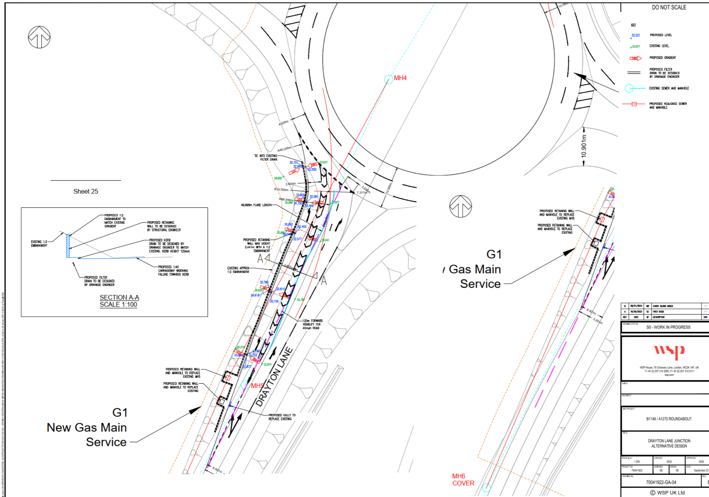
Figure 2 A1270/Drayton Lane Junction - Southern Arm Emerging NCC Capacity Enhancement Scheme
